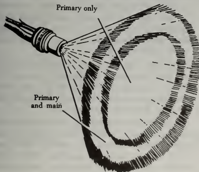
FIGURE 3-60. Duplex nozzle spray pattern.
